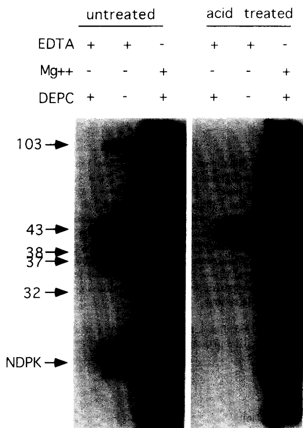
Fig. 2. DEPC abolishes cellular phosphorylation. Cytoplasmic brain extracts, either untreated or treated with DEPC, were phosphorylated in the presence of EDTA at 4°C or MgCl_2 at 30°C, separated, blotted and exposed as described in Fig. 1. The membrane was then treated with 50 mM KCl-HCl (pH 1) (acid treated) and re-exposed.
